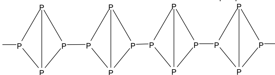
Red phosphorus
