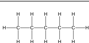
pentane
