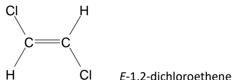
E-1,2-dichloroethene
