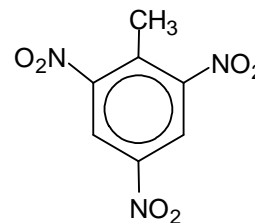
2,4,6-trinitrotoluene
