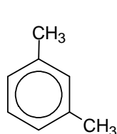
1,3-dimethylbenzene
