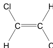
E-1,2-dichloroethene
