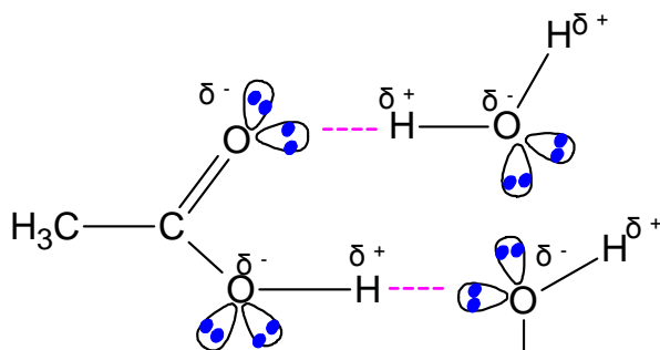
Hydrogen bonding between ethanoic acid and water
